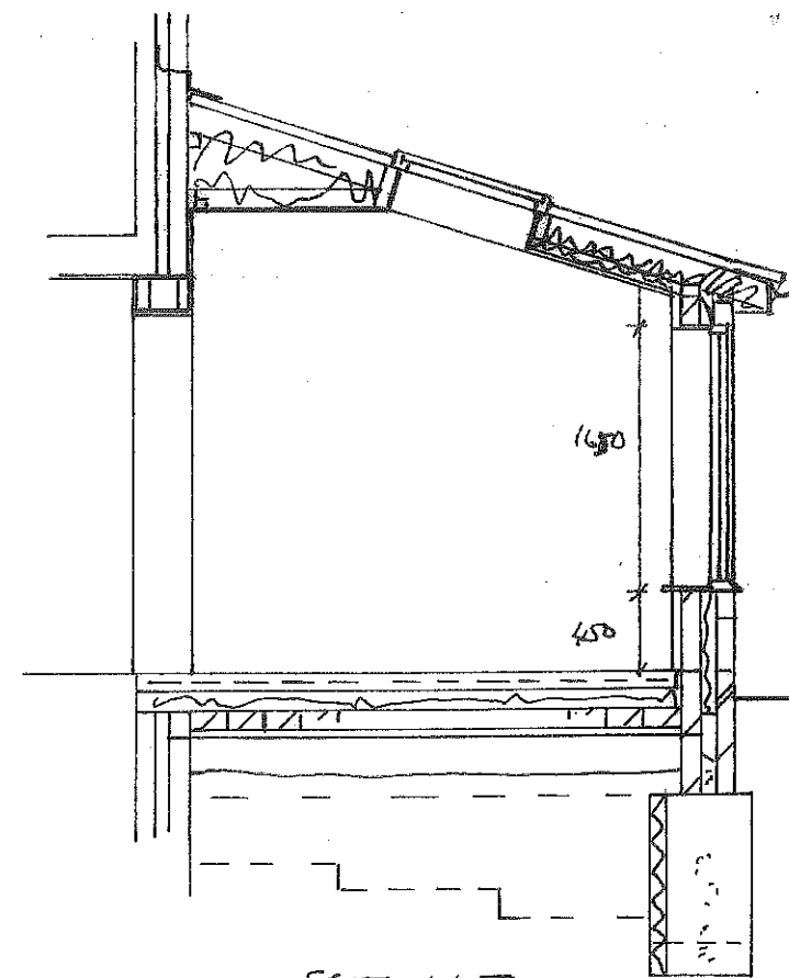
SECTION 1:50
